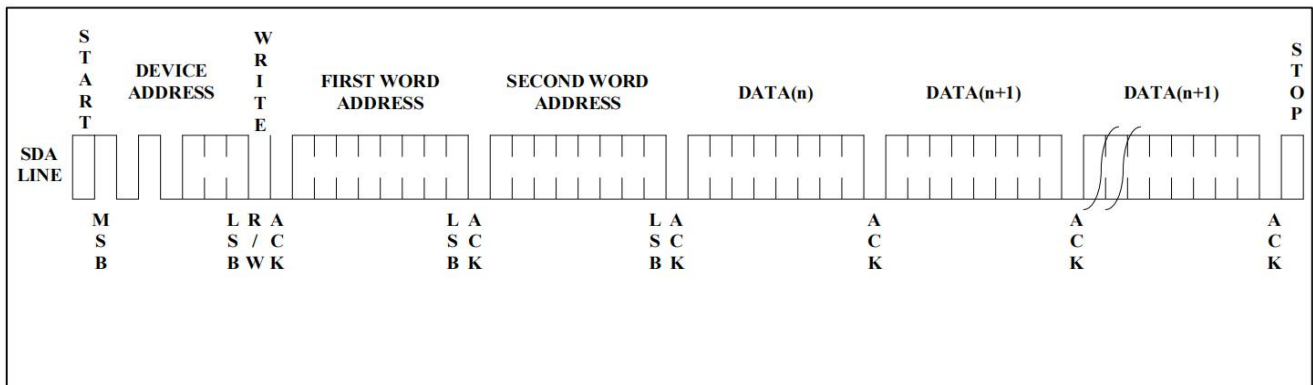
Figure 7. Page Write
