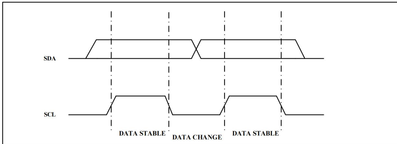
Figure 2. Data Validity
