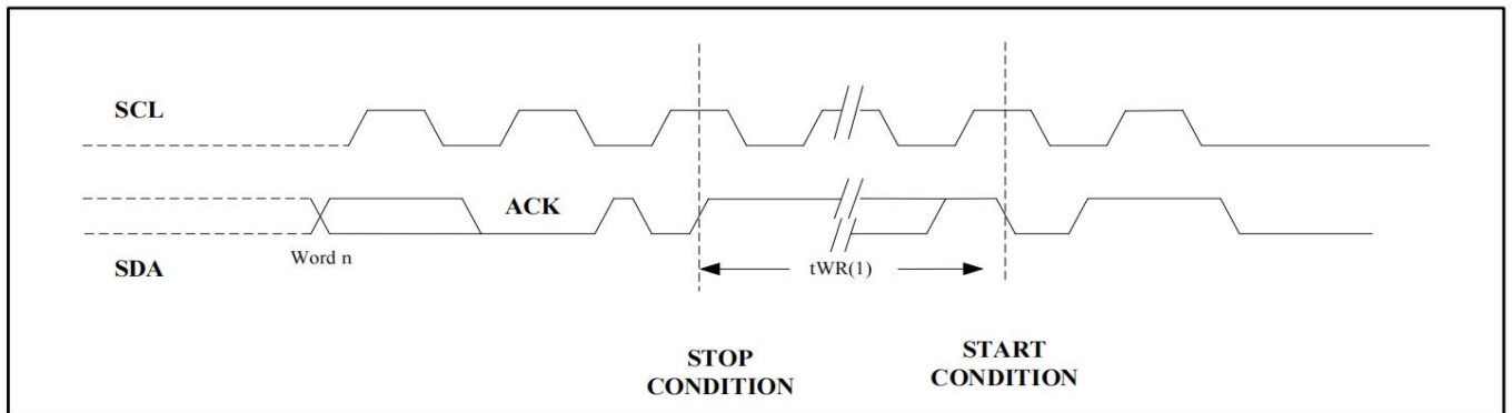
Figure 12. SCL: Serial Clock, SDA: Serial Data I/O
