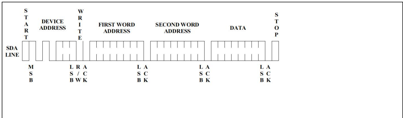
Figure 6. Byte Write
