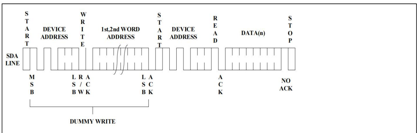
Figure 9. Random Read
