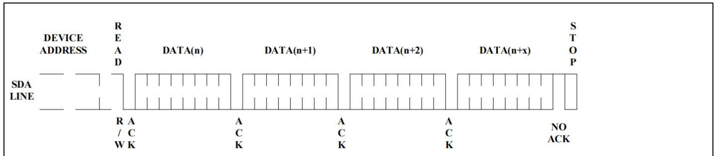
Figure 10. Sequential Read
