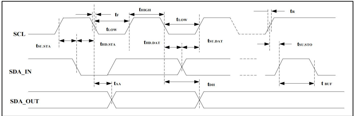
Figure 11. SCL: Serial Clock, SDA: Serial Data I/O
