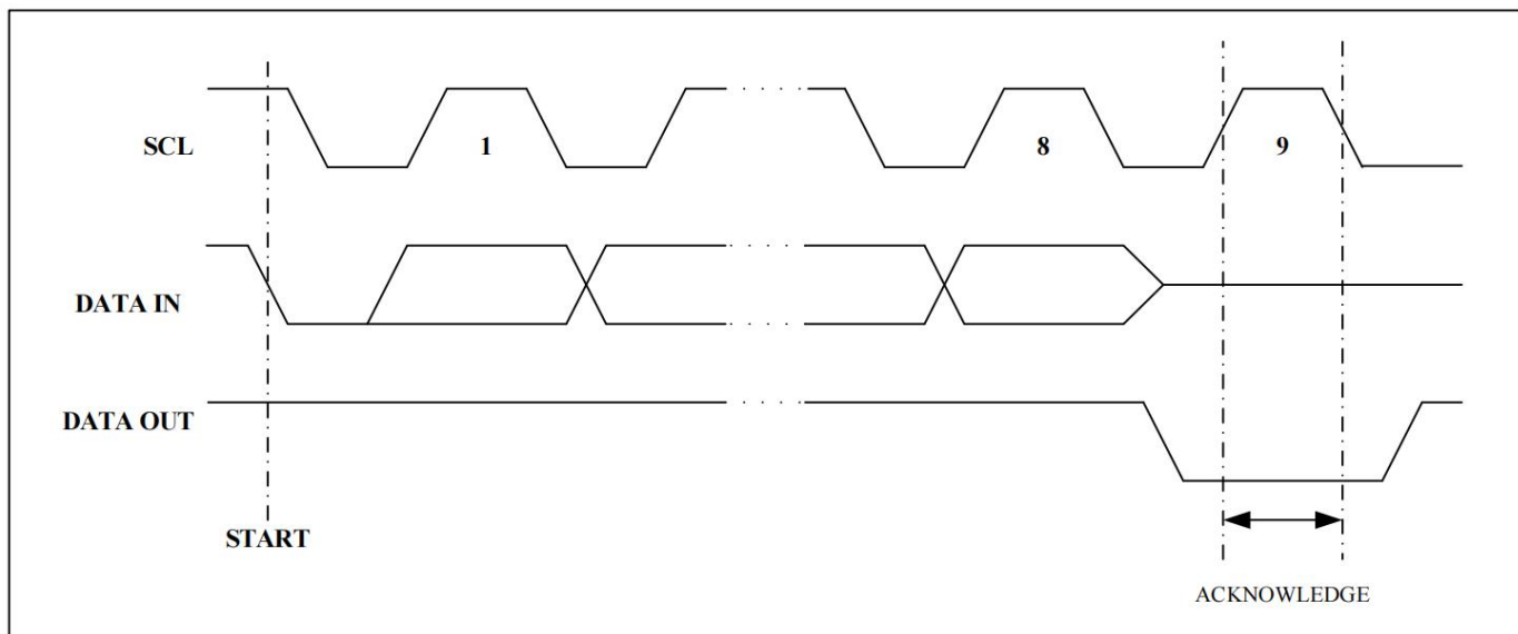
Figure 4. Output Acknowledge
