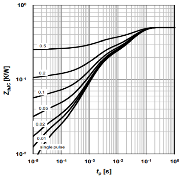
Max. transient thermal impedance Z_{thJC}=f(t_p)
