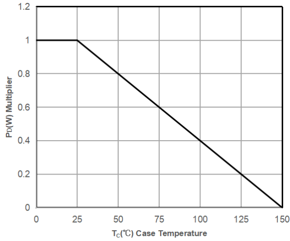
Power Dissipation P_{tot}=f(T_c)
