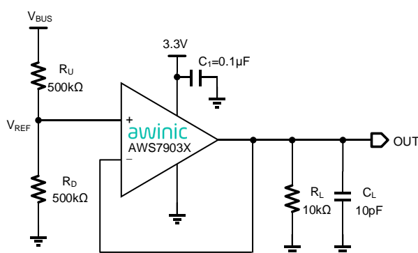
Figure 1 Typical Application of AWS7903X
