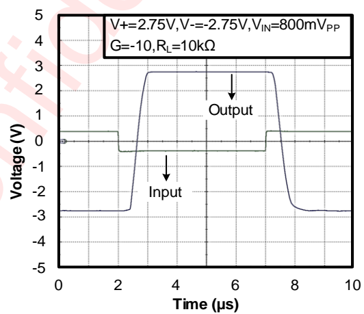
Figure 26 Overload Recovery
