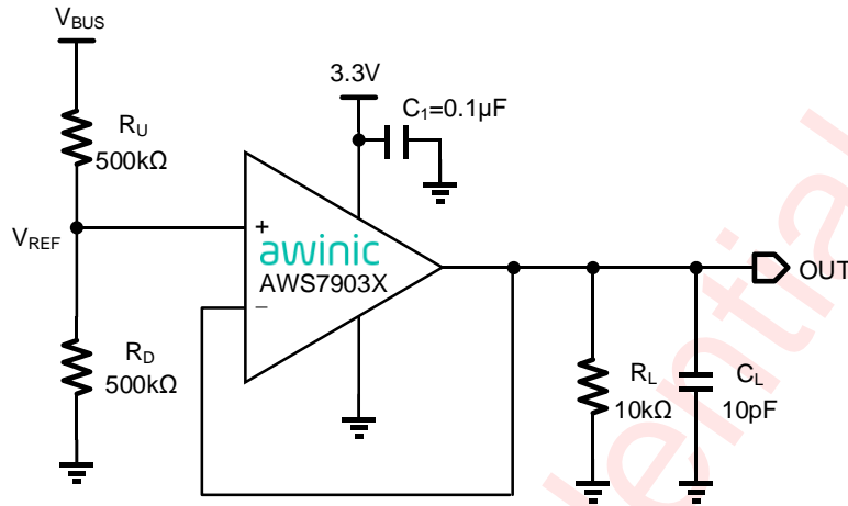
Figure 4 AWS7903X Application Circuit
