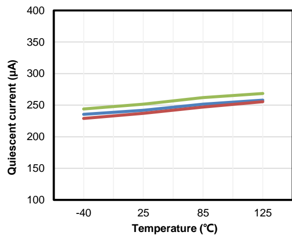
Figure 22 IQ vs. Temperature
