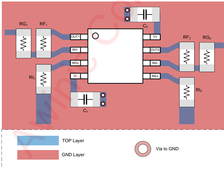
Figure 38 AWS7903X Layout Example
