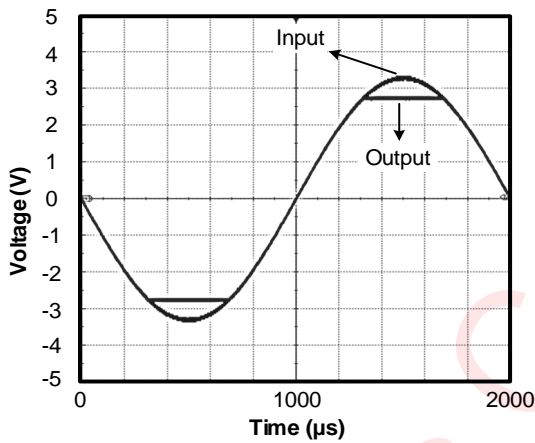
Figure 25 No Phase Reversal
