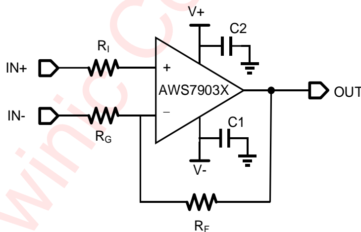
Figure 37 AWS7903X Schematic Example
