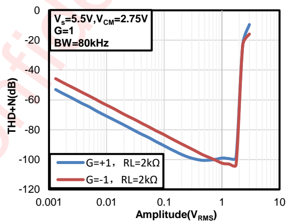
Figure 20 THD+N vs. Amplitude
