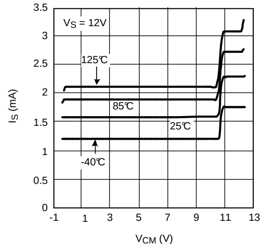
Figure 14. I_S vs V_{CM}
