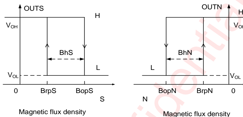
Figure 4 The Working Process of AW86503DNR
