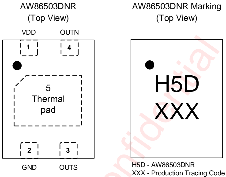
Figure 2 Pin Configuration and Top Mark
