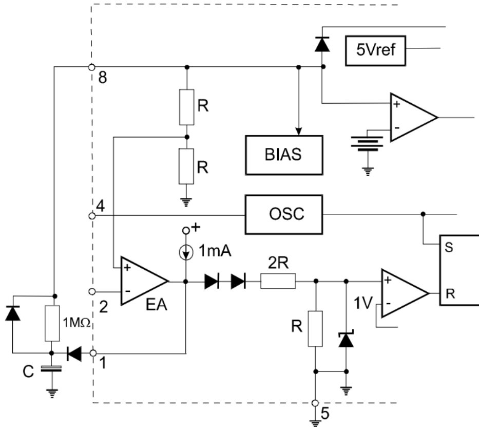
Figure 8. Soft-Start Circuit
