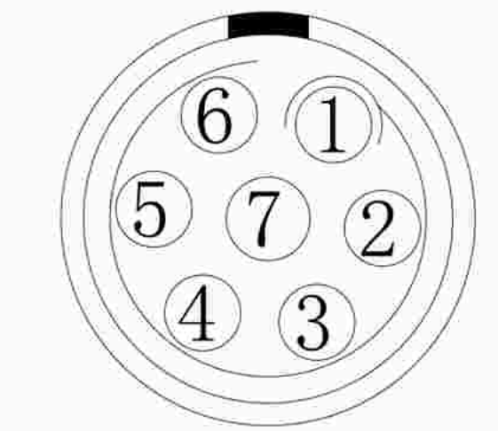
Welded surface (焊接面)
