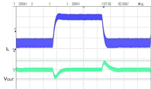
(16) Load Transient(VIN=50.0V,VOUT=12V,IOUT=0.1→0.6A)
