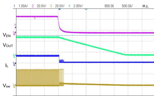
(18) Enable Shutdown(VIN=30.0V,VOUT=3.3V,IOUT=0.6A)
