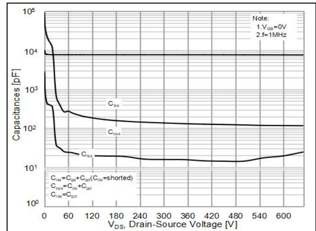
Figure10. Capacitance
