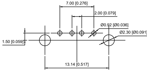
PCB LAYOUT XKB Connectivity
