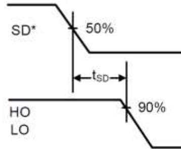
Figure 2. Shutdown Waveform Definition
