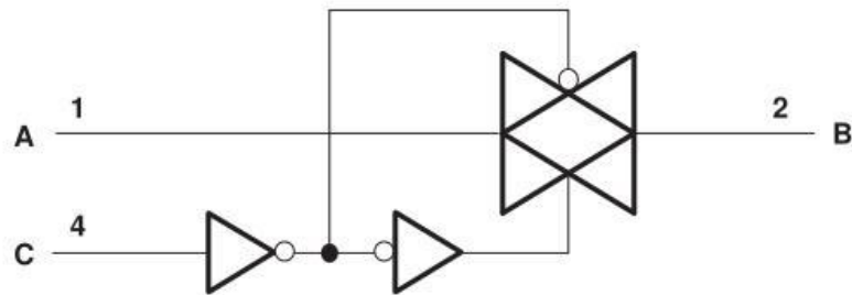
Figure 3.1: 74LVC1G66Gx,125 Logic Diagram
