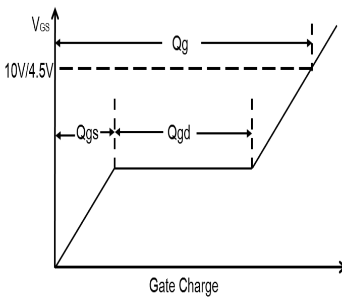
Fig.8 Gate Charge Waveform
