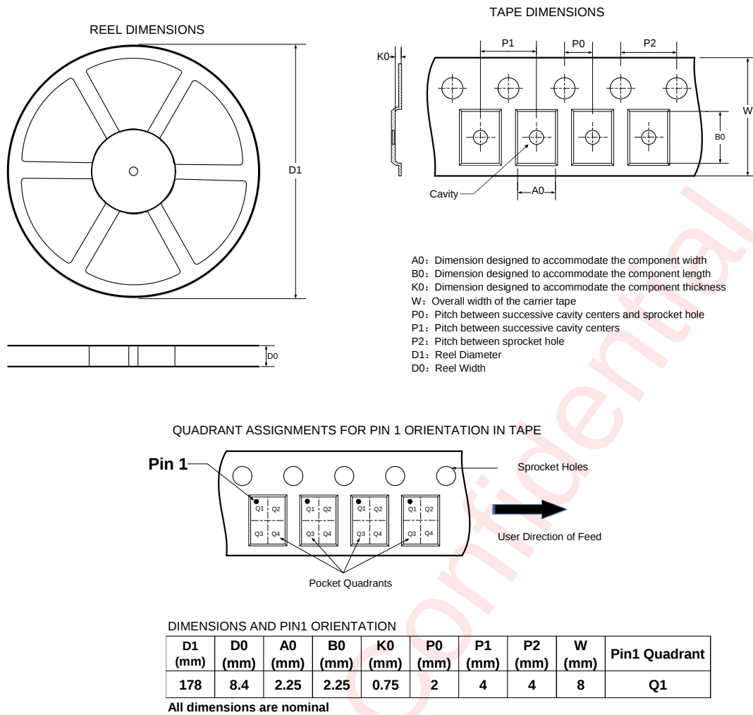
Figure 5 Tape and Reel
