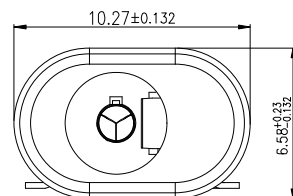
O-Ring assembly state
