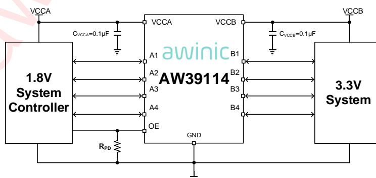
Figure 1 Typical Application Circuit of AW39114
