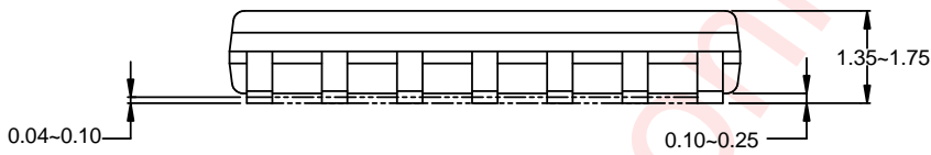
SIDE VIEW
