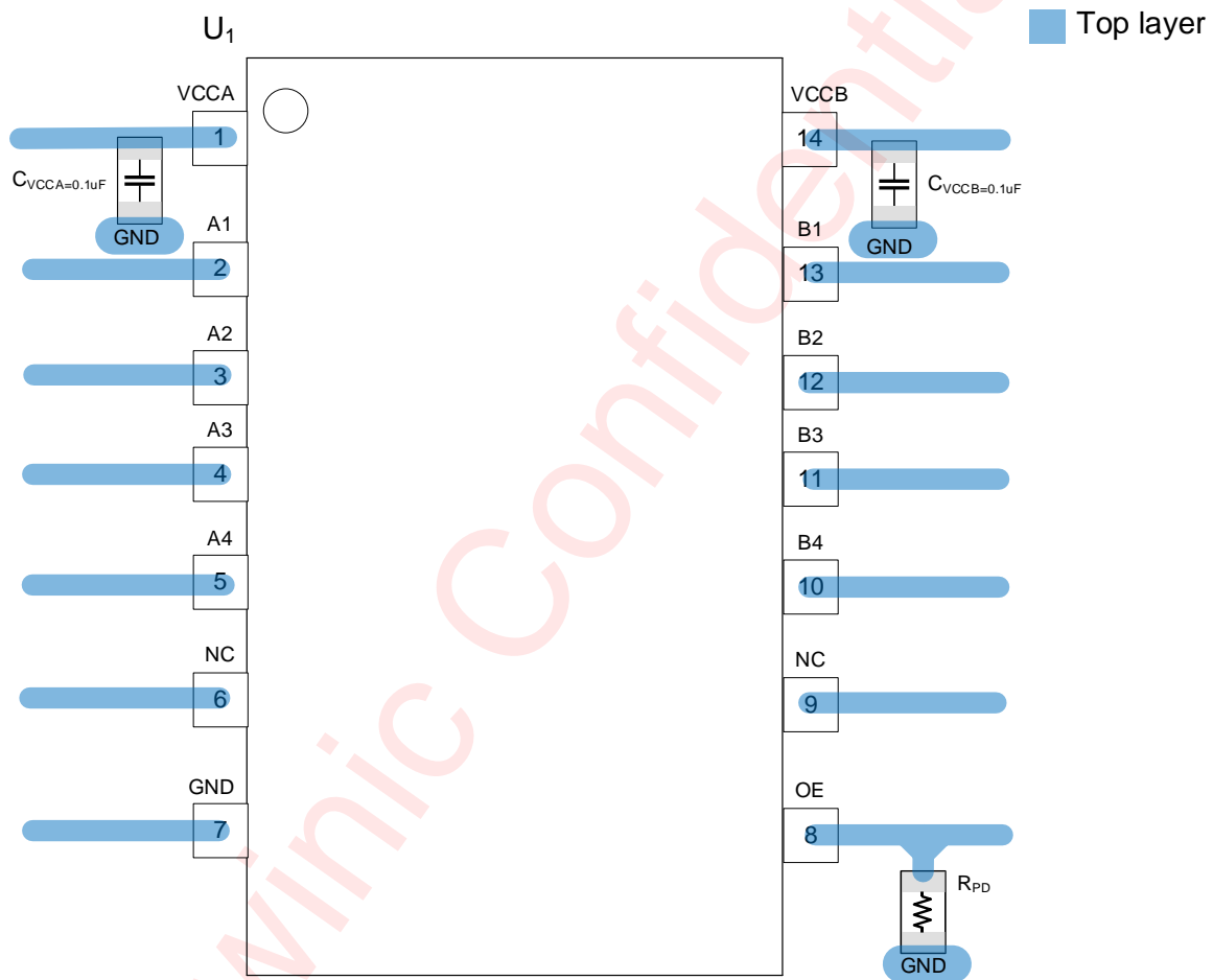
Figure 15 AW39114SPR Layout Example
