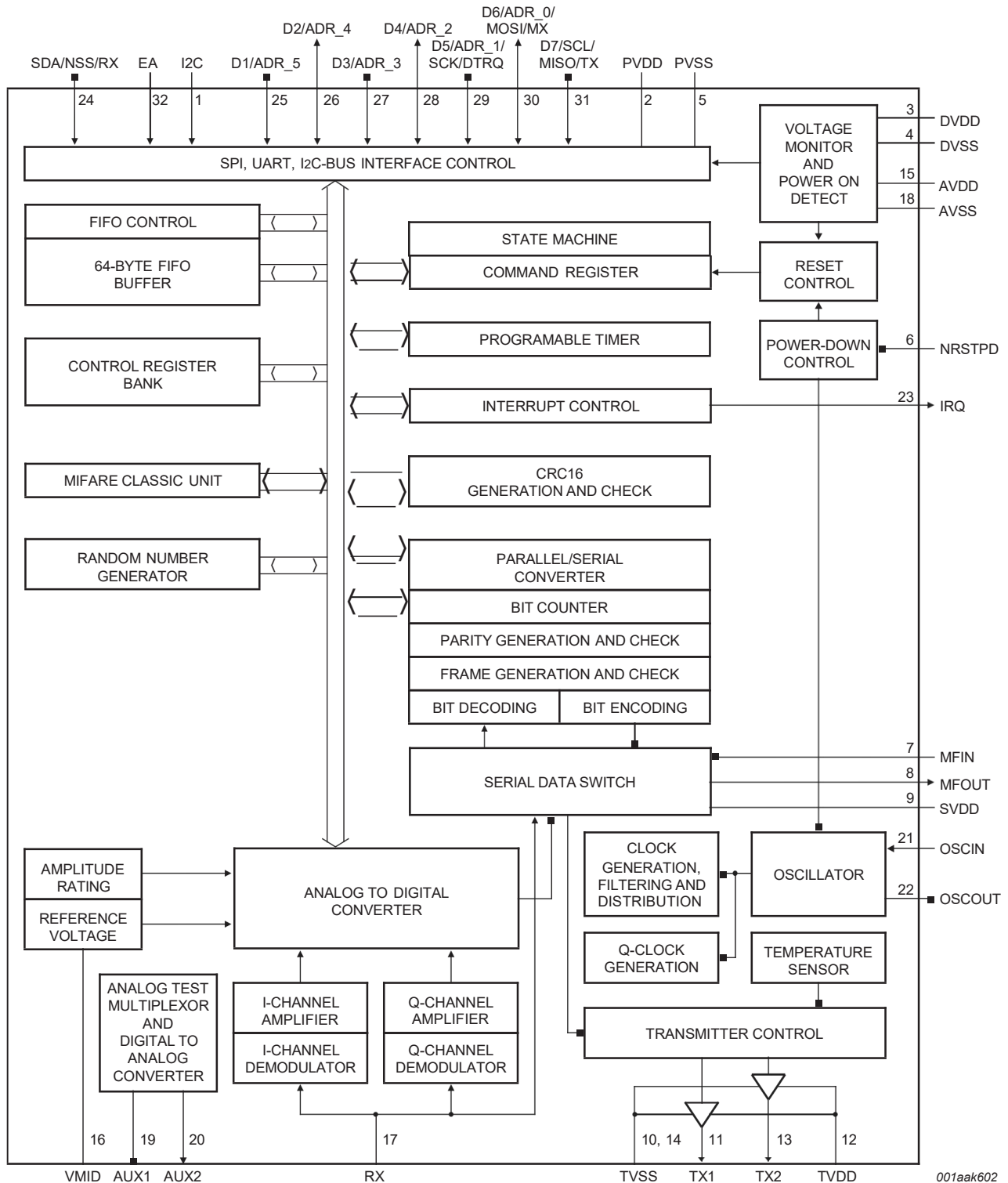
Fig 2. Detailed block diagram of the HX523-Q
