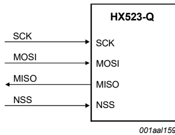
Fig 7. SPI connection to host
