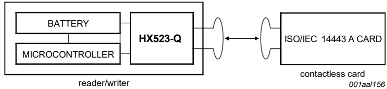
Fig 4. HX523-Q Read/Write mode
