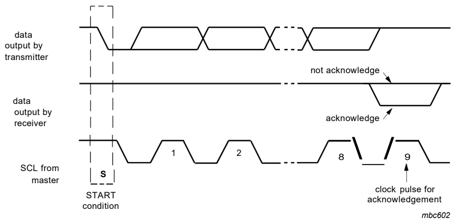
Fig 14. Acknowledge on the I2C-bus
