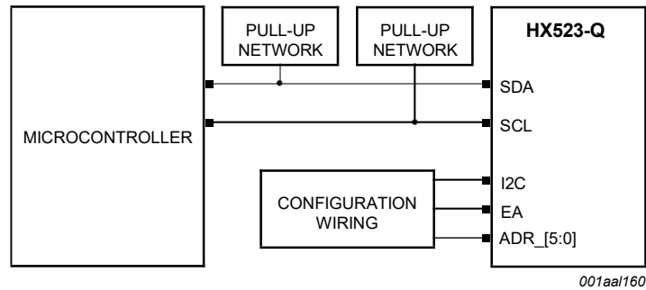
Fig 11. I2C-bus interface
