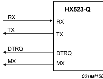
Fig 8. UART connection to microcontrollers
