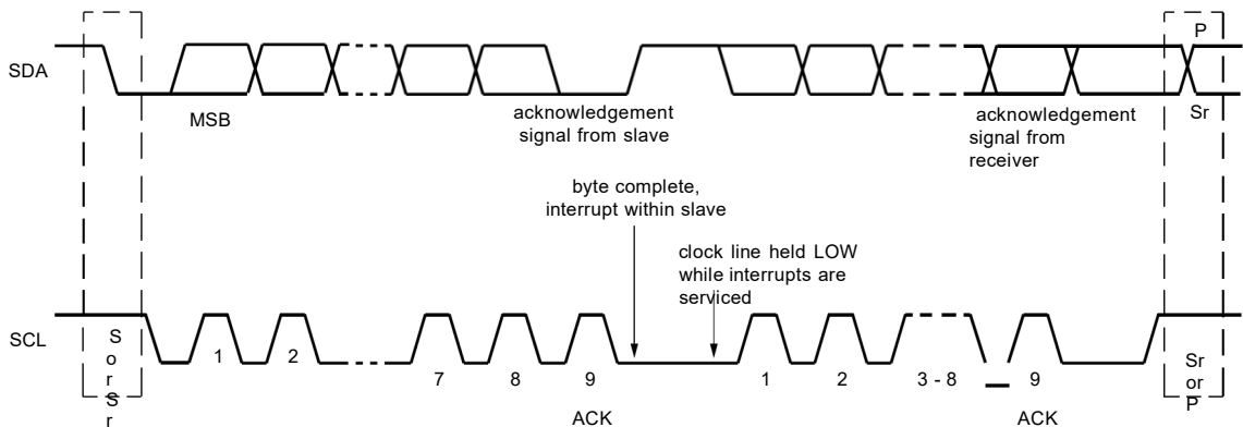
Fig 15. Data transfer on the I2C-bus
