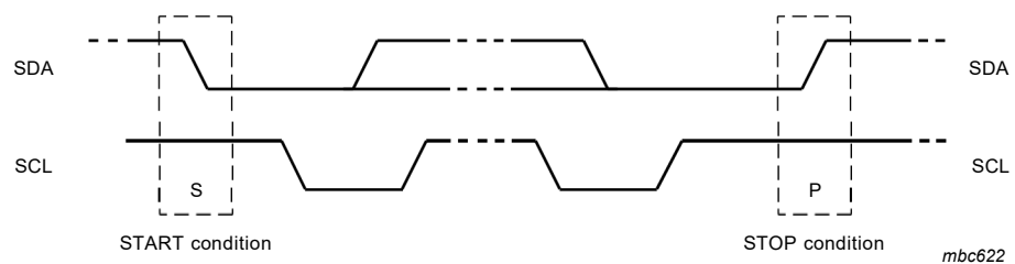
Fig 13. START and STOP conditions
