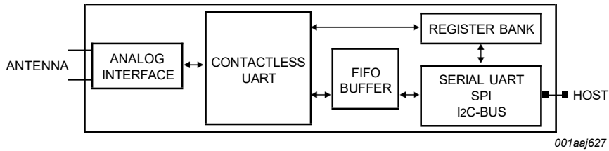
Fig 1. Simplified block diagram of the HX523-Q
