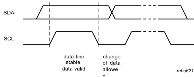
Fig 12. Bit transfer on the I2C-bus
