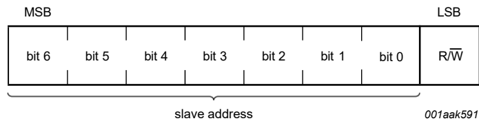
Fig 16. First byte following the START procedure
