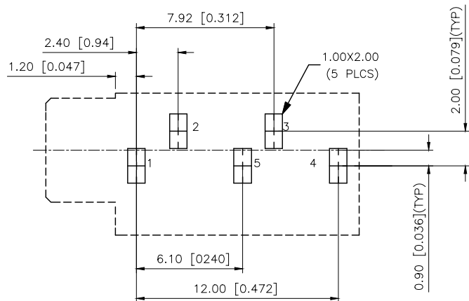
PCB Layout
