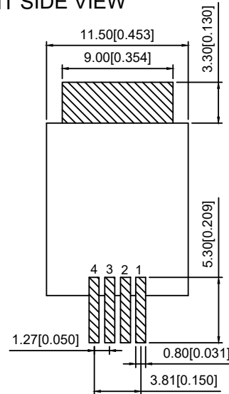
RECOMMENDED PCB LAYOUT VIEWED FROM COMPONENT SIDE
