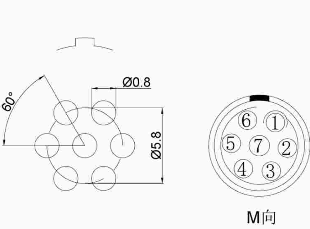
Pcb plate opening size (PCB板开孔尺寸)
