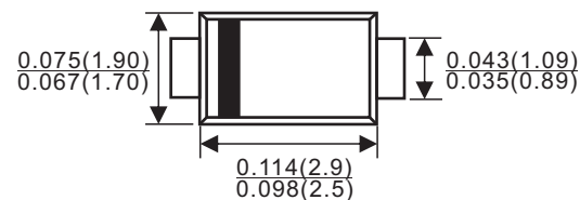
SOD-123FL
