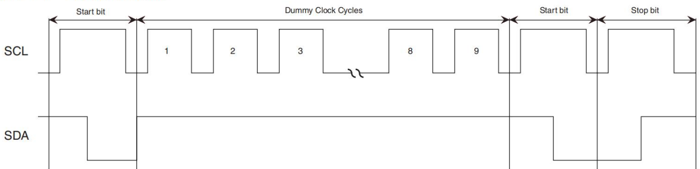
Figure 4-1. Software Reset
