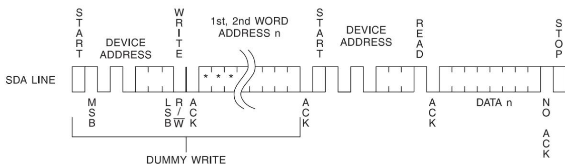
Figure 12-5. Random Read
