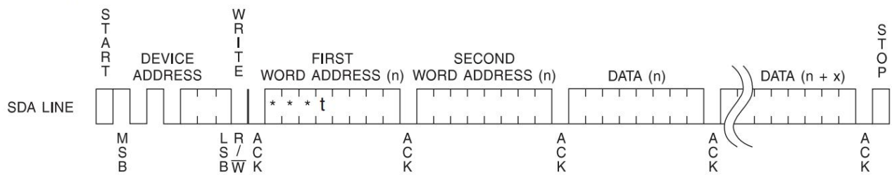
Figure 12-3. Page Write
