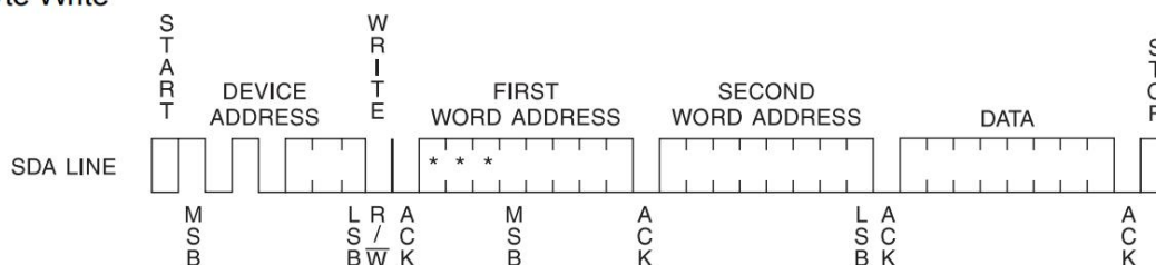
Figure 12-2. Byte Write
