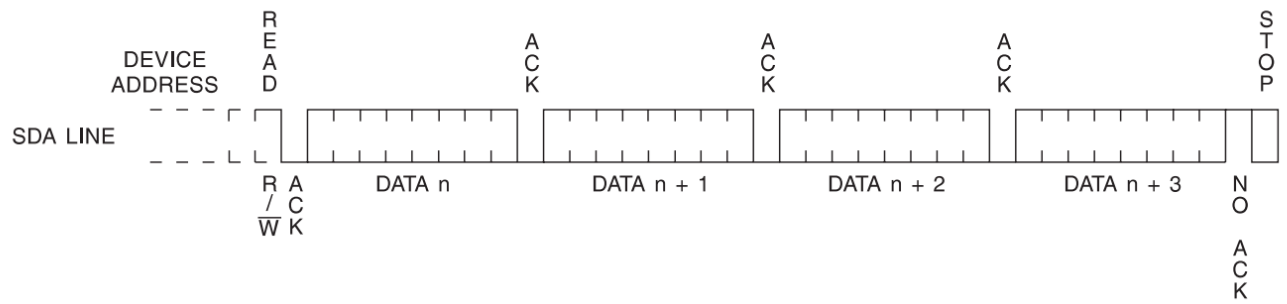
Figure 12-6. Sequential Read
