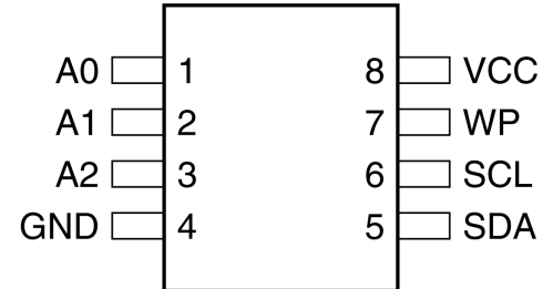
8-lead SOIC
