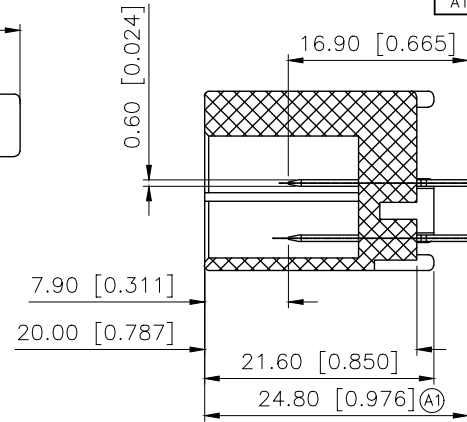
SECTION:A-A SCALE:1:1
