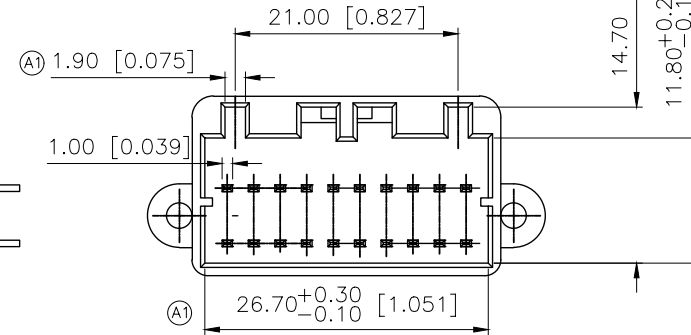
SECTION:A-A SCALE:1:1
