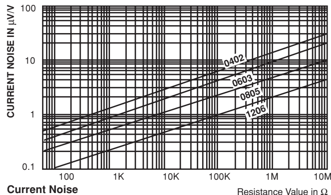
Current Noise
