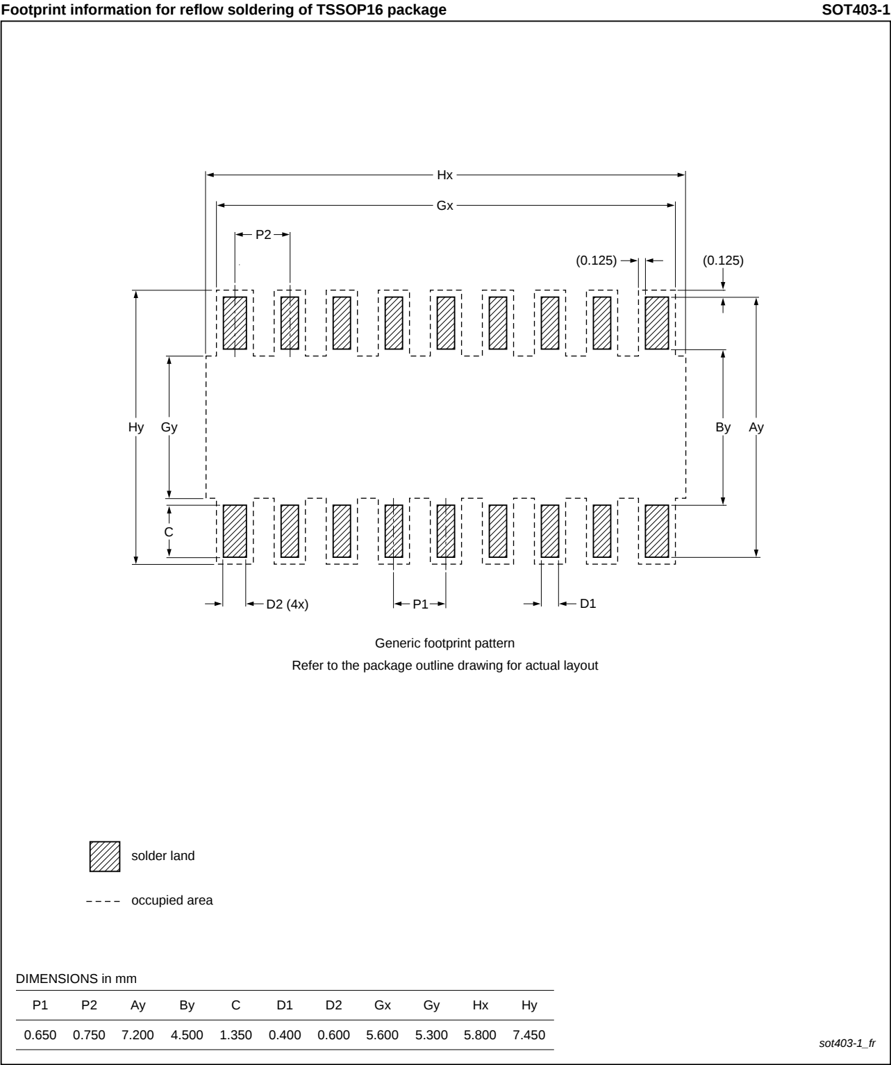
Fig 19. PCB footprint for SOT403-1 (TSSOP16); reflow soldering
