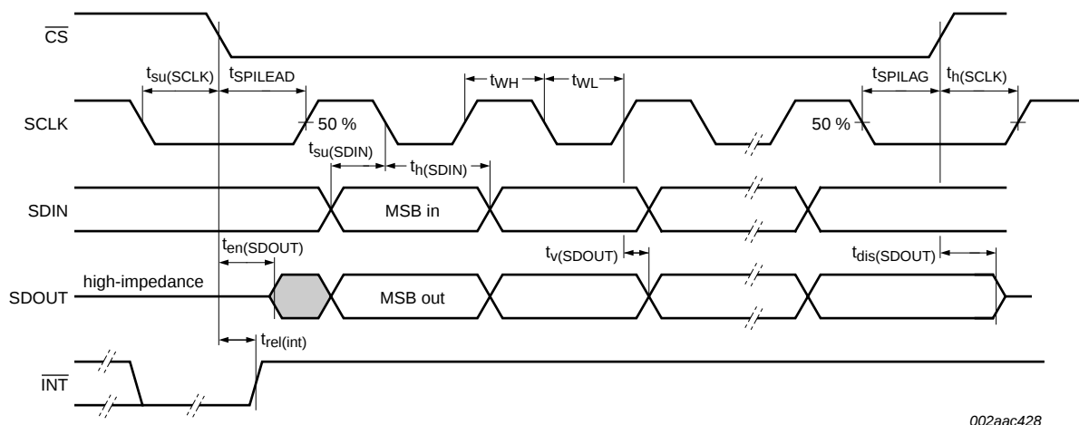
Fig 11. Timing diagram
