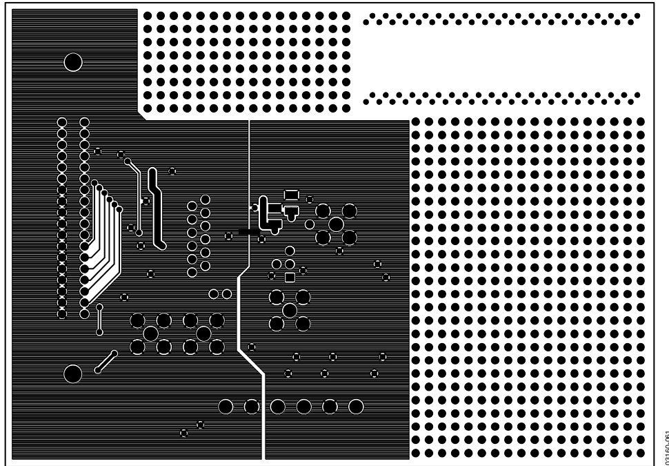
Figure 62. Solder-Side Artwork
