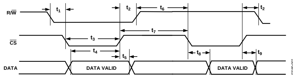
Figure 2. Timing Diagram
