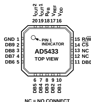
Figure 6. AD5433 Pin Configuration (LFCSP).
