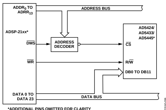
Figure 56. ADSP21xx-to-AD5424/AD5433/AD5445 Interface
