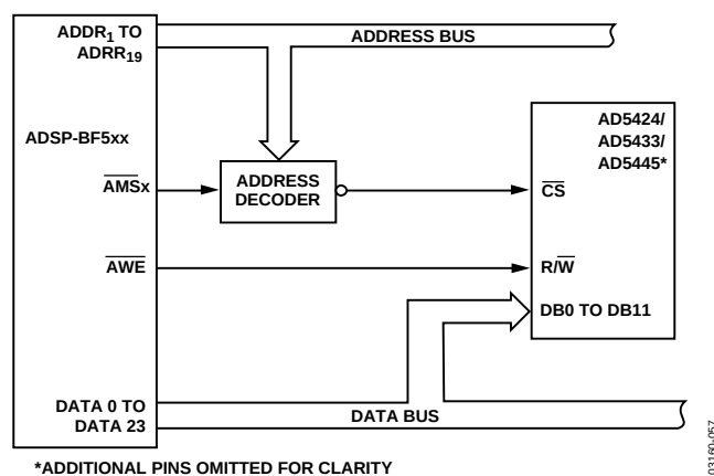
Figure 58. ADSP-BF5xx-to-AD5424/AD5433/AD5445 Interface
