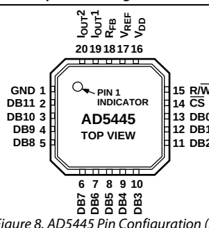
Figure 8. AD5445 Pin Configuration (LFCSP)
