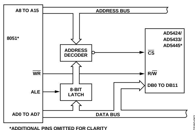
Figure 57. 8xC51-to-AD5424/AD5433/AD5445 Interface
