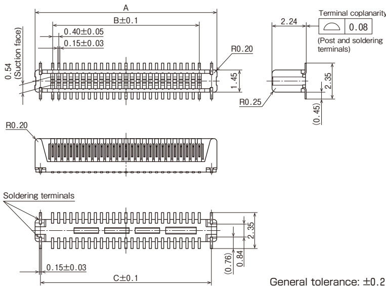
Dimension table
