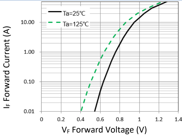
Figure 1. Forward Characteristic(typ.)
