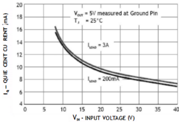
QUIESCENT CURRENT
