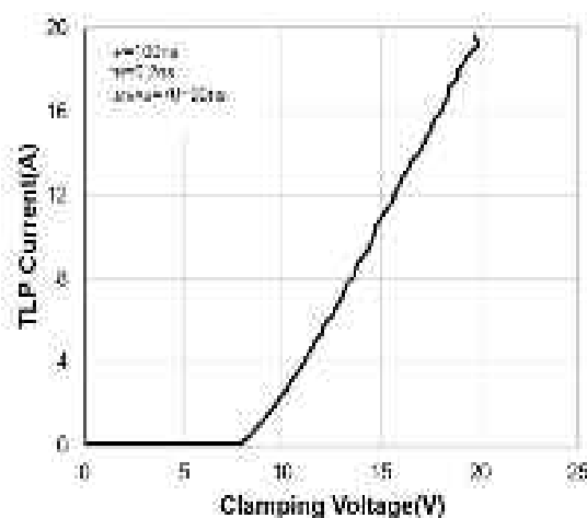
TLP Curve
