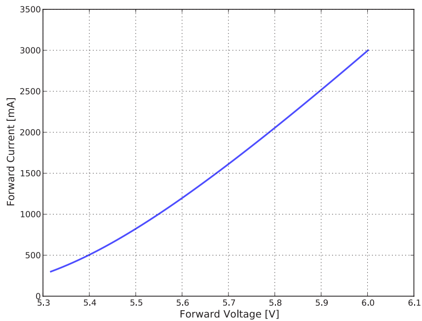
Figure 5b. Typical forward current vs. forward voltage for L1MX-xxxx06Vxxxxx0 at Tj=85°C.
