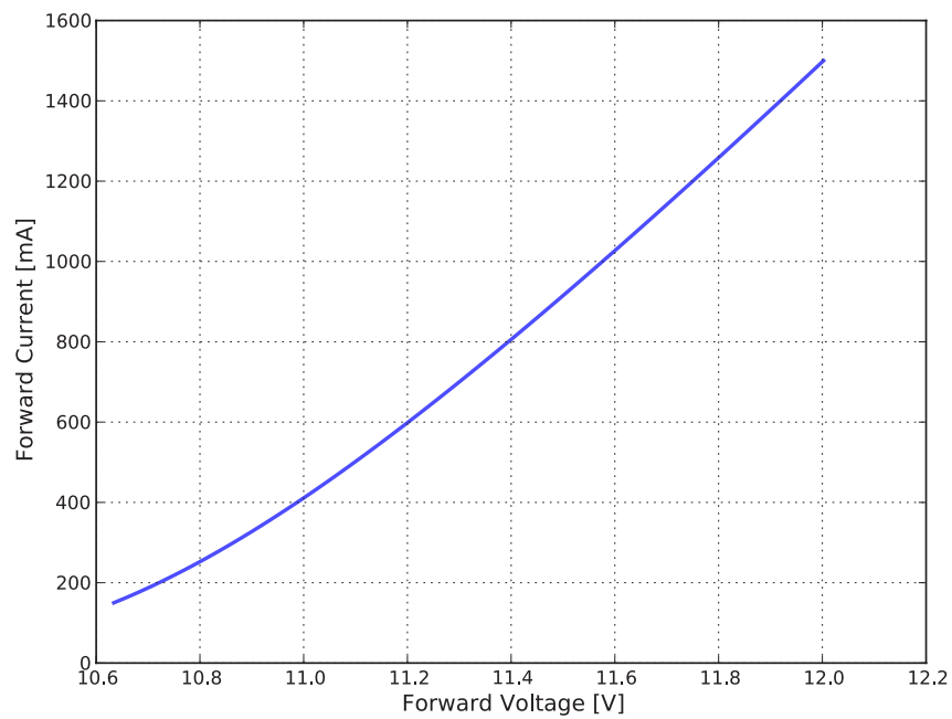
Figure 5a. Typical forward current vs. forward voltage for L1MX-xxxx12Vxxxxx0 at Tj=85°C.
