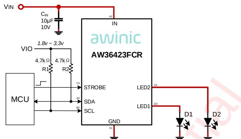
Fig 3 AW36423 Application Circuit
