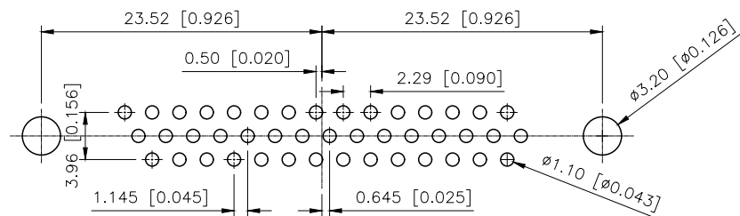
PCB LAYOUT
