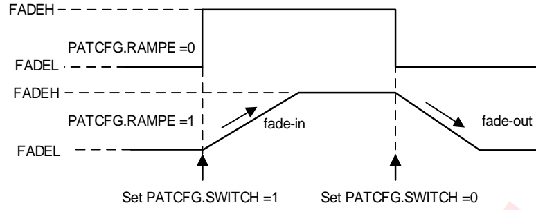
Figure 15 Manual Control Mode
