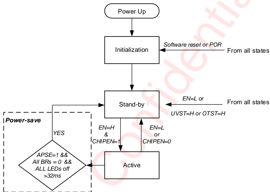
Figure 8 AW21036 Operating Mode Transition
