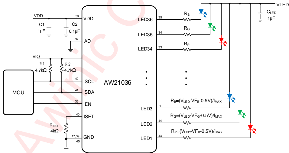
Figure 4 AW21036 Typical Application Circuit
