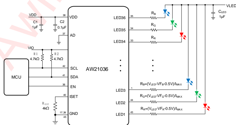
Figure 1 AW21036 Application Circuit
