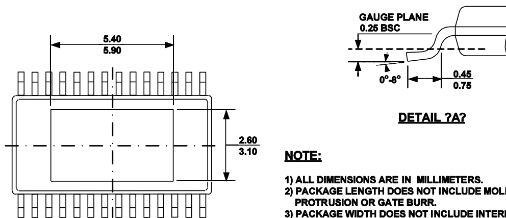
BOTTOM VIEW
