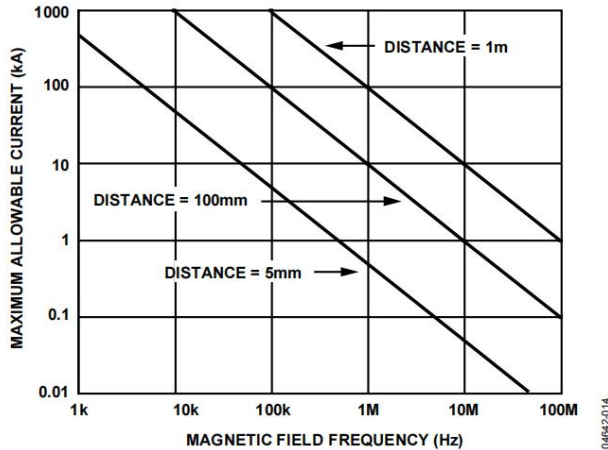
Figure 14. Maximum Allowable Current for Various Current-to-ADuM1200/ADuM1201 Spacings
