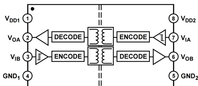
Figure 2. ADuM1201 Functional Block Diagram
