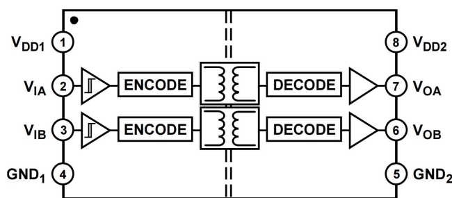
Figure 1. ADuM1200 Functional Block Diagram
