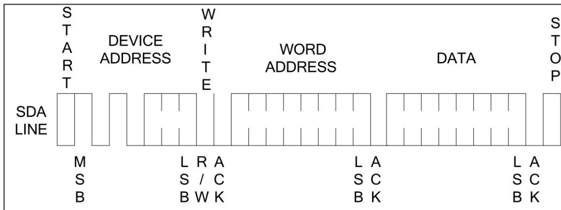
Figure 7. Page Write
