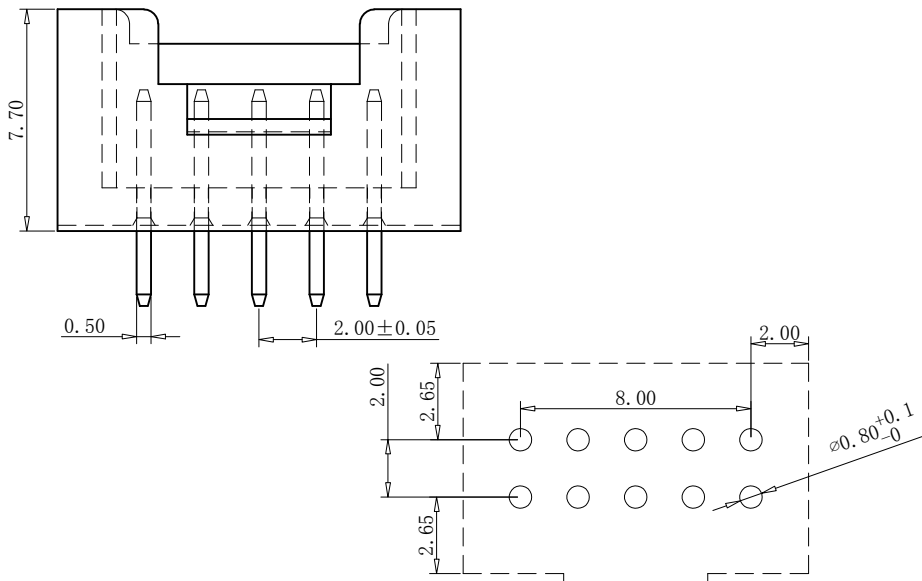
PCB LAYOUT
