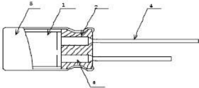
Fig. 1 Cross-section view
