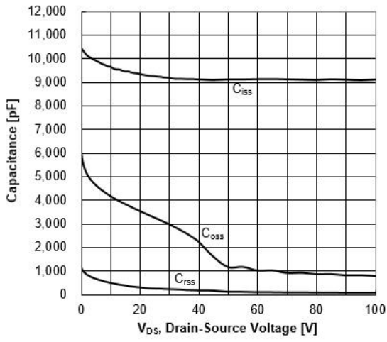
Figure 12. Capacitance Characteristics
