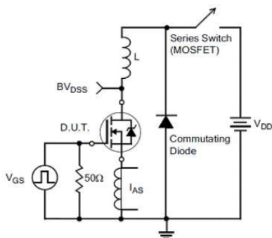
Figure 20. Unclamped Inductive Switching Test Circuit
