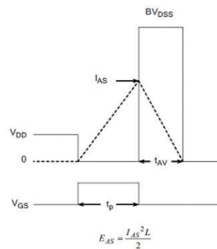
Figure 21. Unclamped Inductive Switching Waveform
