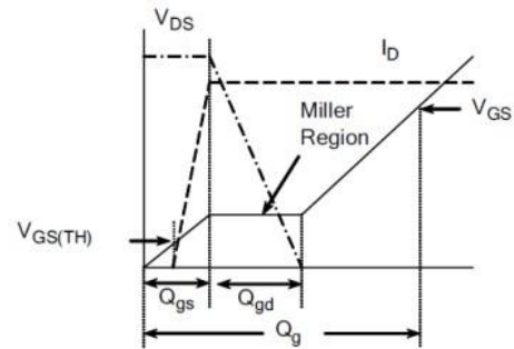
Figure 17. Gate Charge Waveforms
