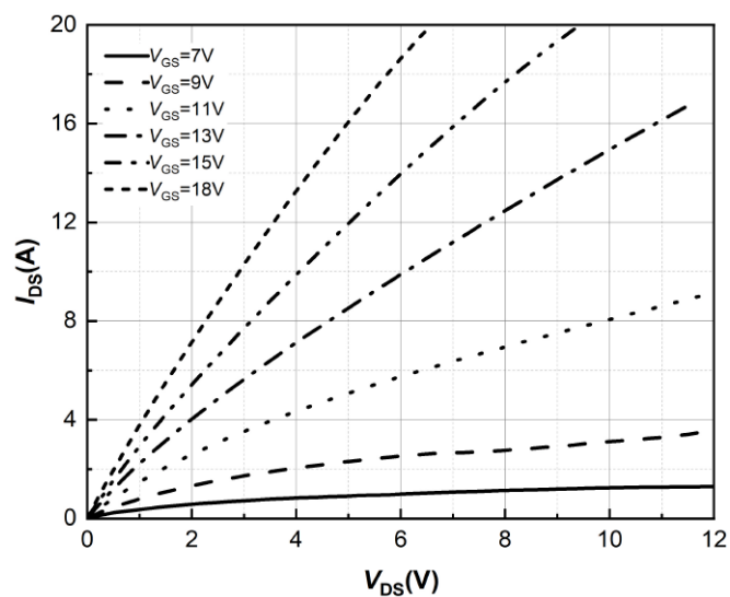
Figure 2 Output Characteristics
