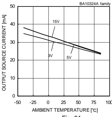
Fig. 31 Output Source Current - Ambient Temperature ( V_{OUT}=0[V] )
