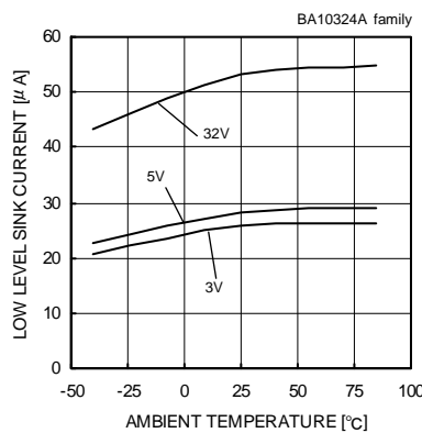
Fig. 35 Low Level Sink Current - Ambient Temperature ( V_{OUT}=0.2[V] )
