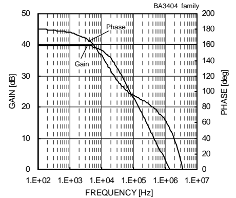
Voltage Gain - Frequency (VCC=±15V)
