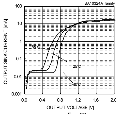
Fig. 32 Output Sink Current - Output Voltage ( V_{CC}=5[V] )
