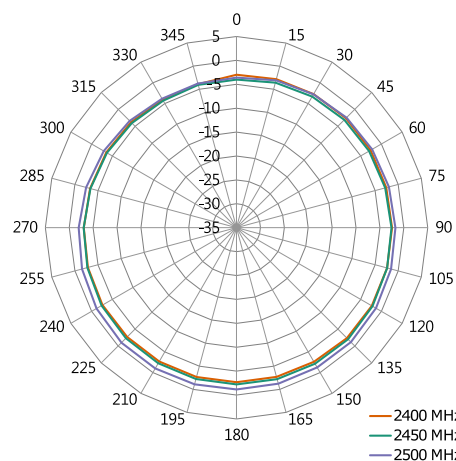
XY-Plane Gain
