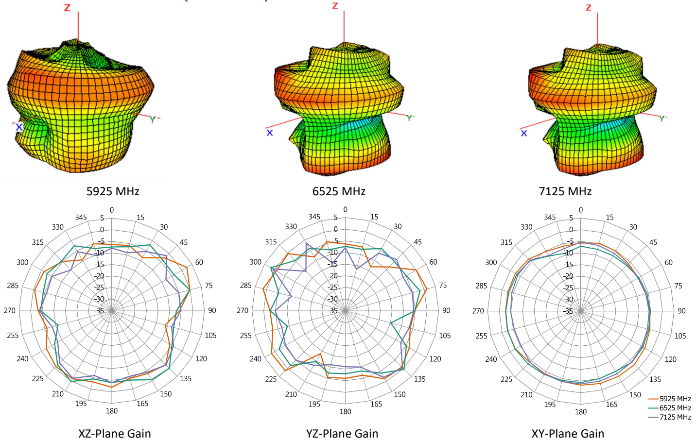
Figure 17-1. Antenna Radiation Patterns, Edge Bent 90 Degrees
