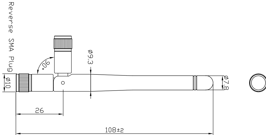
Figure 2. Antenna Dimensions
