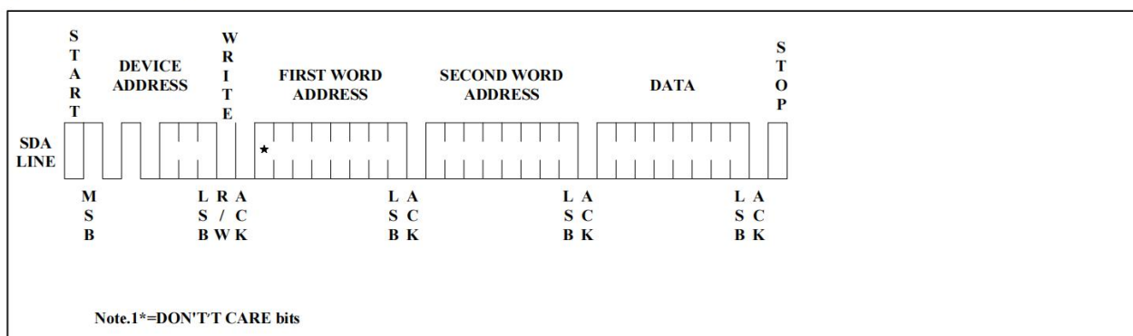
Figure 6. Byte Write
