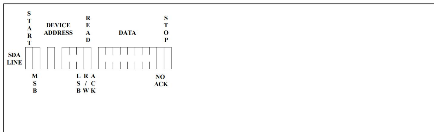
Figure 9. Random Read
