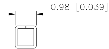
SECTION:C-C SCALE:1:1
