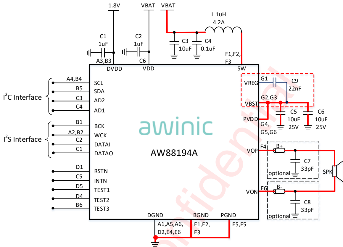
Figure 3 AW88194A Application Circuit
