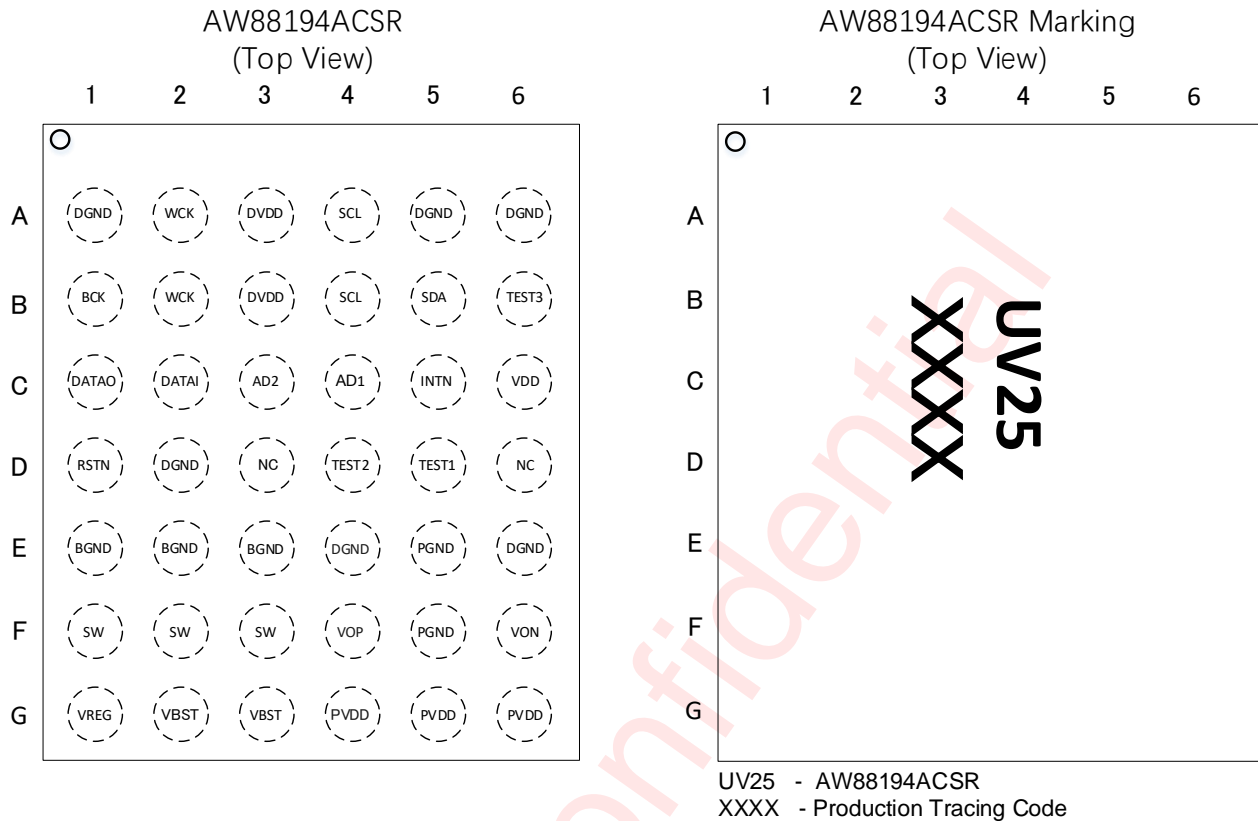
Figure 1 AW88194ACSR pin diagram top view and device marking
