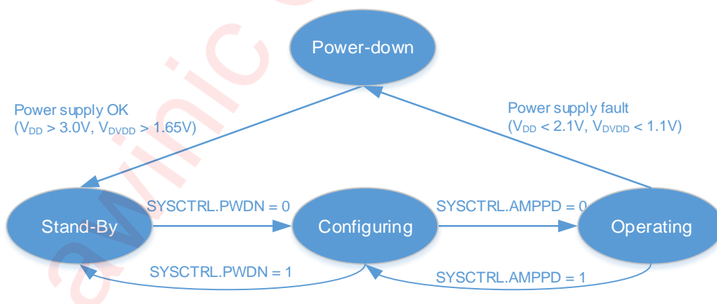
Figure 7 Device operating modes transition
