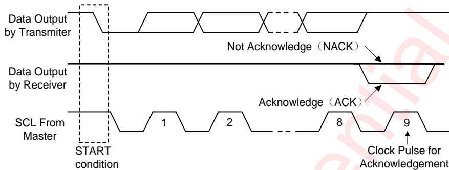
Figure 22 I 2 C ACK Timing
