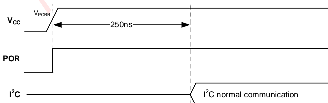
Figure 15 Power On Timing
