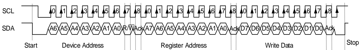
Figure 23 I 2 C Write Byte Cycle
