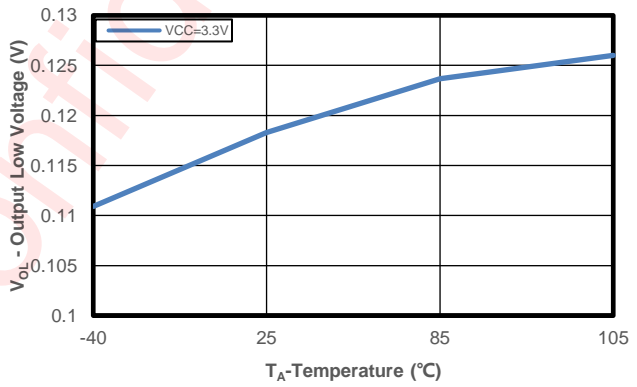
Figure 9 AW9535/AW9555 GPIO Output Low Voltage VS Temperature
