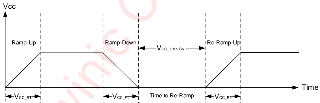
Figure 31 V_{CC} is Lowered Below 0.2V or 0V and Then Ramped Up to V_{CC}
