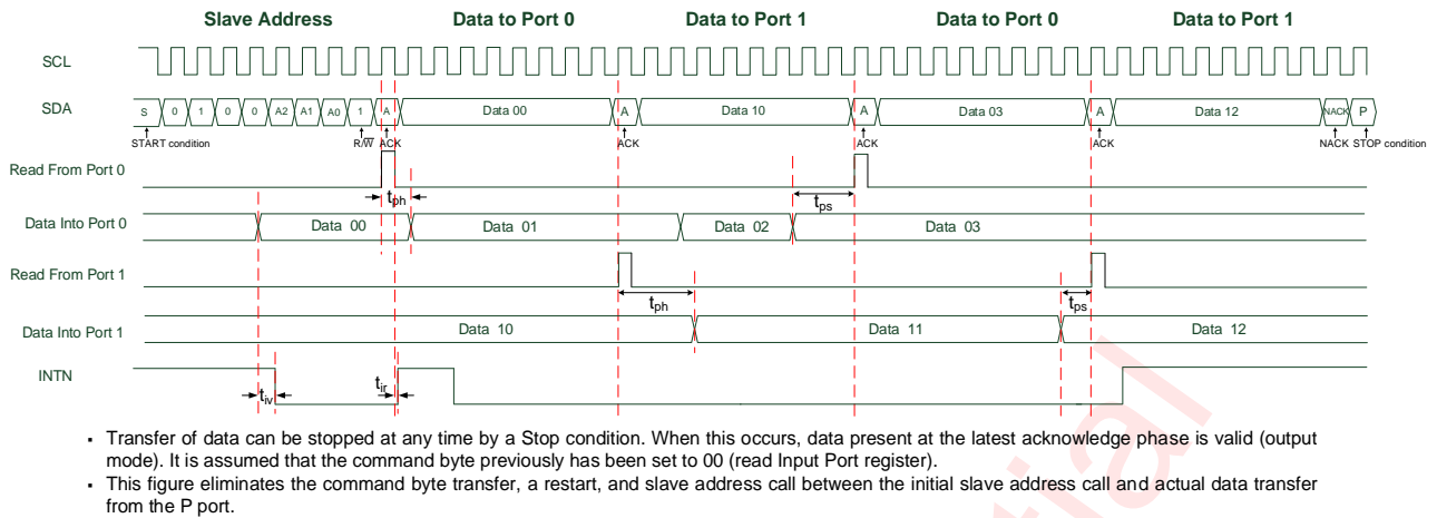
Figure 19 Read Input Port Register, Scenario 2
