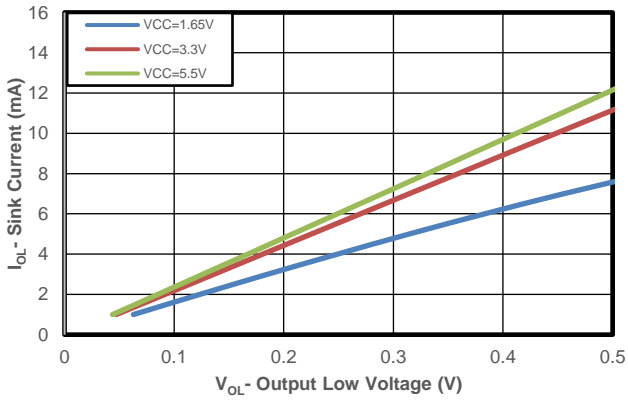
Figure 12 AW9535/AW9555 INTN Pin Output Low Voltage VS INTN Current for Different V_{CC}
