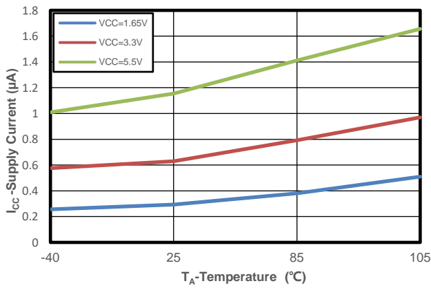
Figure 6 AW9535 Standby Supply Current (P port= V_{CC} or GND) and AW9555 Standby Supply Current (P port= V_{CC} ) VS Temperature for Different Supply Voltage ( V_{CC} )
