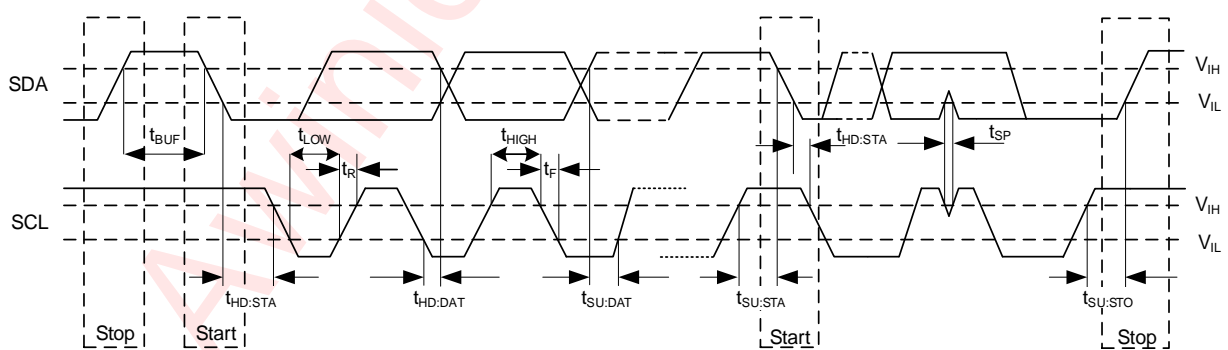
Figure 4 Definition of Timing on The I 2 C-bus
