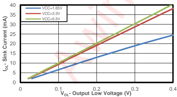
Figure 10 AW9535/AW9555 P Port Output Low Voltage VS Current for Different V_{CC}
