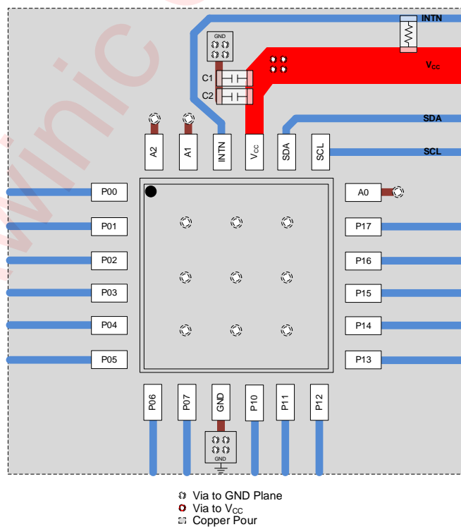
Figure 36 AW9535QNR Layout Example
