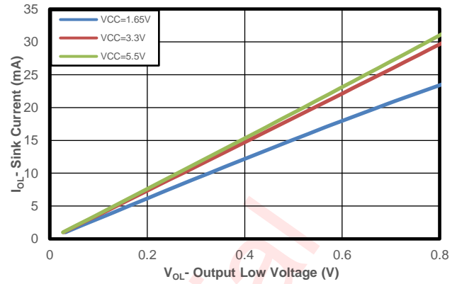
Figure 13 AW9535/AW9555 SDA Pin Output Low Voltage VS SDA Current for Different V_{CC}
