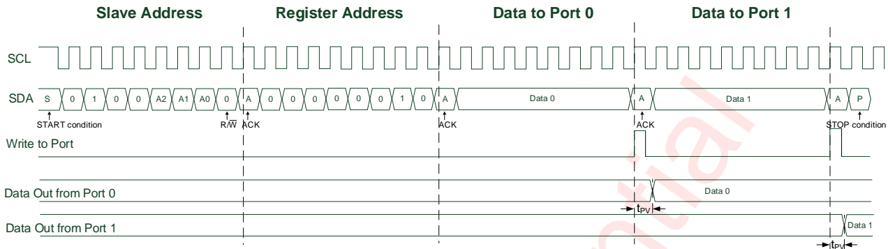
Figure 17 Write to Output Port Registers
