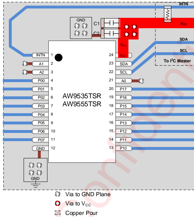
Figure 35 AW9535TSR/AW9555TSR Layout Example
