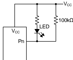
Figure 27 High-Value Resistor in Parallel With LED
