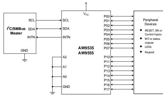
Figure 1 AW9535/AW9555 Simplified Application Circuit
