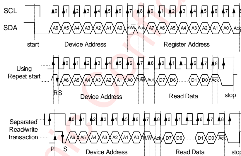
Figure 24 I 2 C Read Byte Cycle
