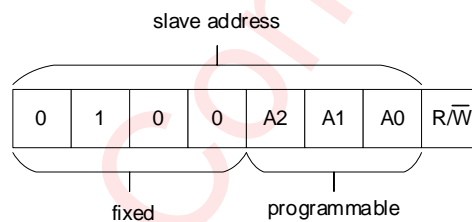
Figure 14 AW9535/AW9555 Device Address
