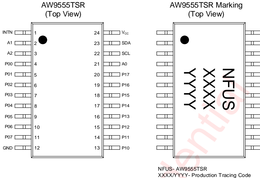
Figure 2 Pin Configuration and Marking
