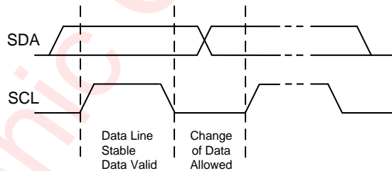
Figure 20 Data Validation Diagram
