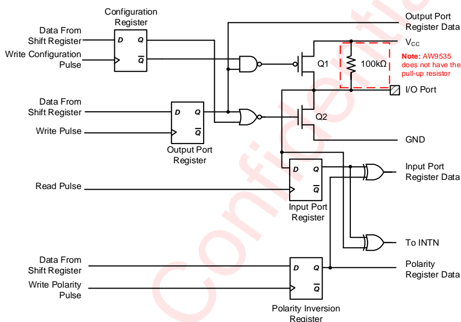
Figure 16 Simplified Schematic of I/Os
