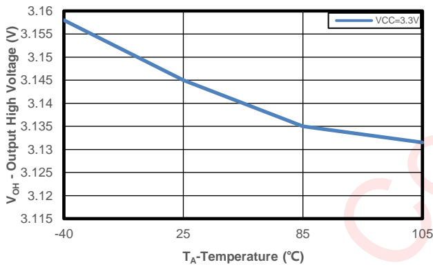
Figure 8 AW9535/AW9555 GPIO Output High Voltage VS Temperature
