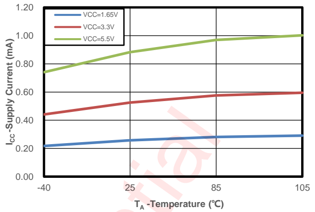
Figure 7 AW9555 Standby Supply Current (P port=GND) VS Temperature for Different Supply Voltage ( V_{CC} )
