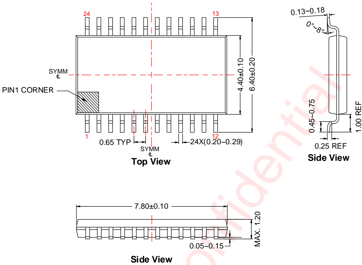
AW9535TSR/AW9555TSR Package Description
