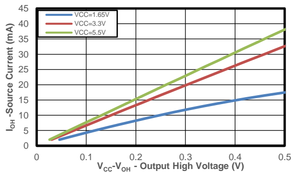
Figure 11 AW9535/AW9555 P Port Output High Voltage VS Current for Different V_{CC}
