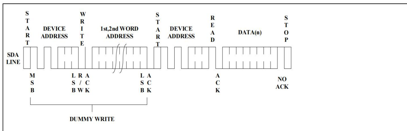
Figure 9. Random Read
