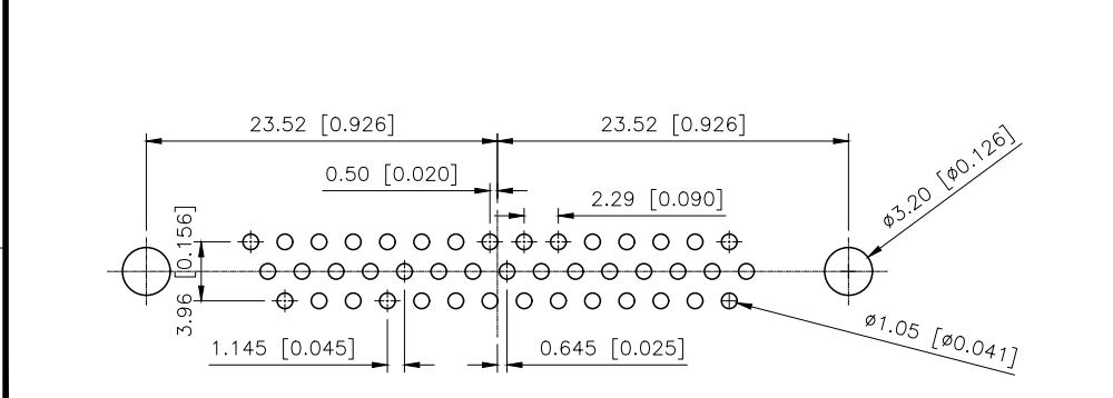
PCB LAYOUT
