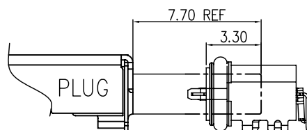
MATING INTERFACE
